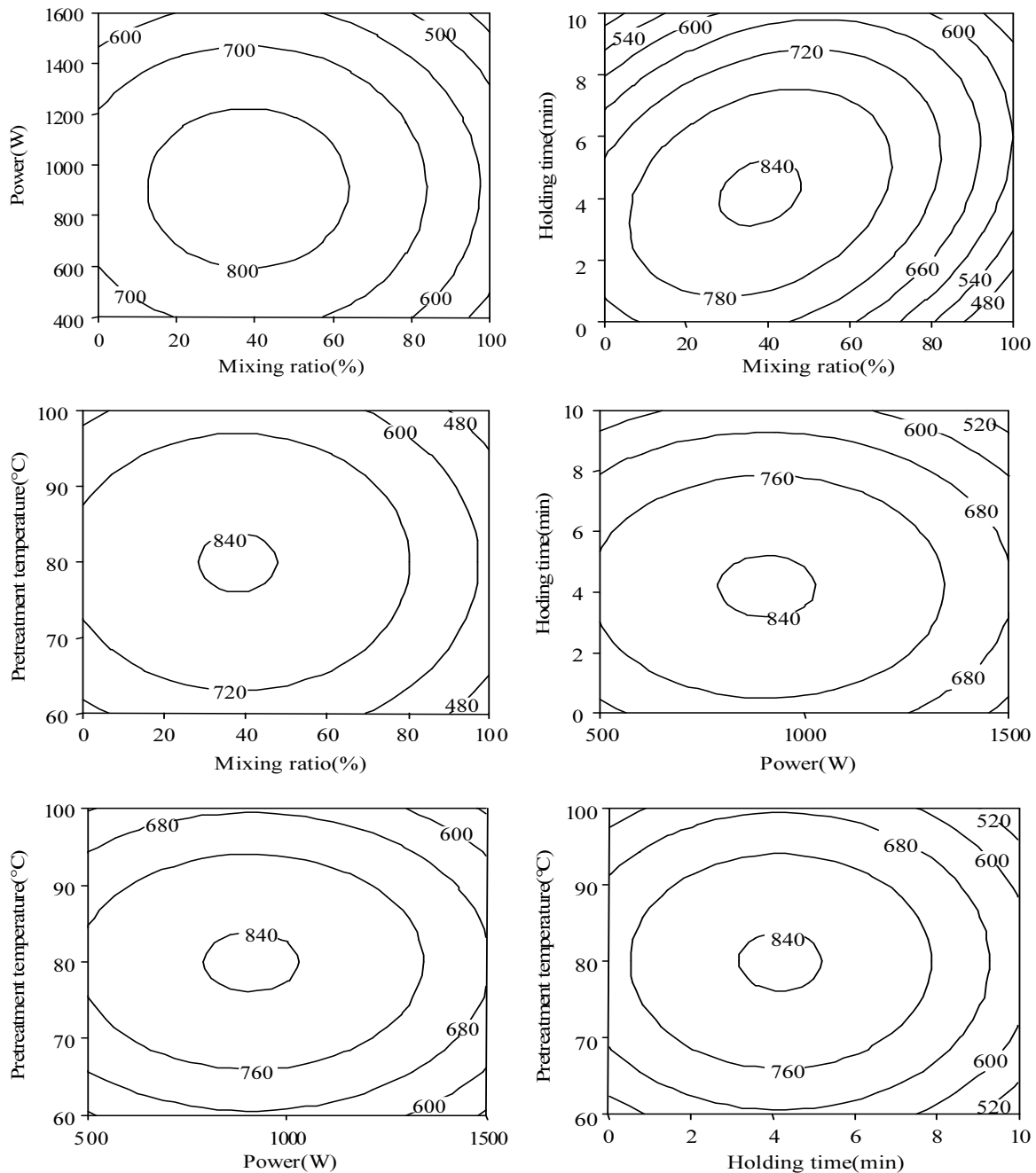
Fig. 6 Two-dimensional contour plot of the quadratic model for methane yield degree of sludge with respect to pretreatment conditions of mixing ration, power, holding time and pretreatment temperature within the design boundaries
